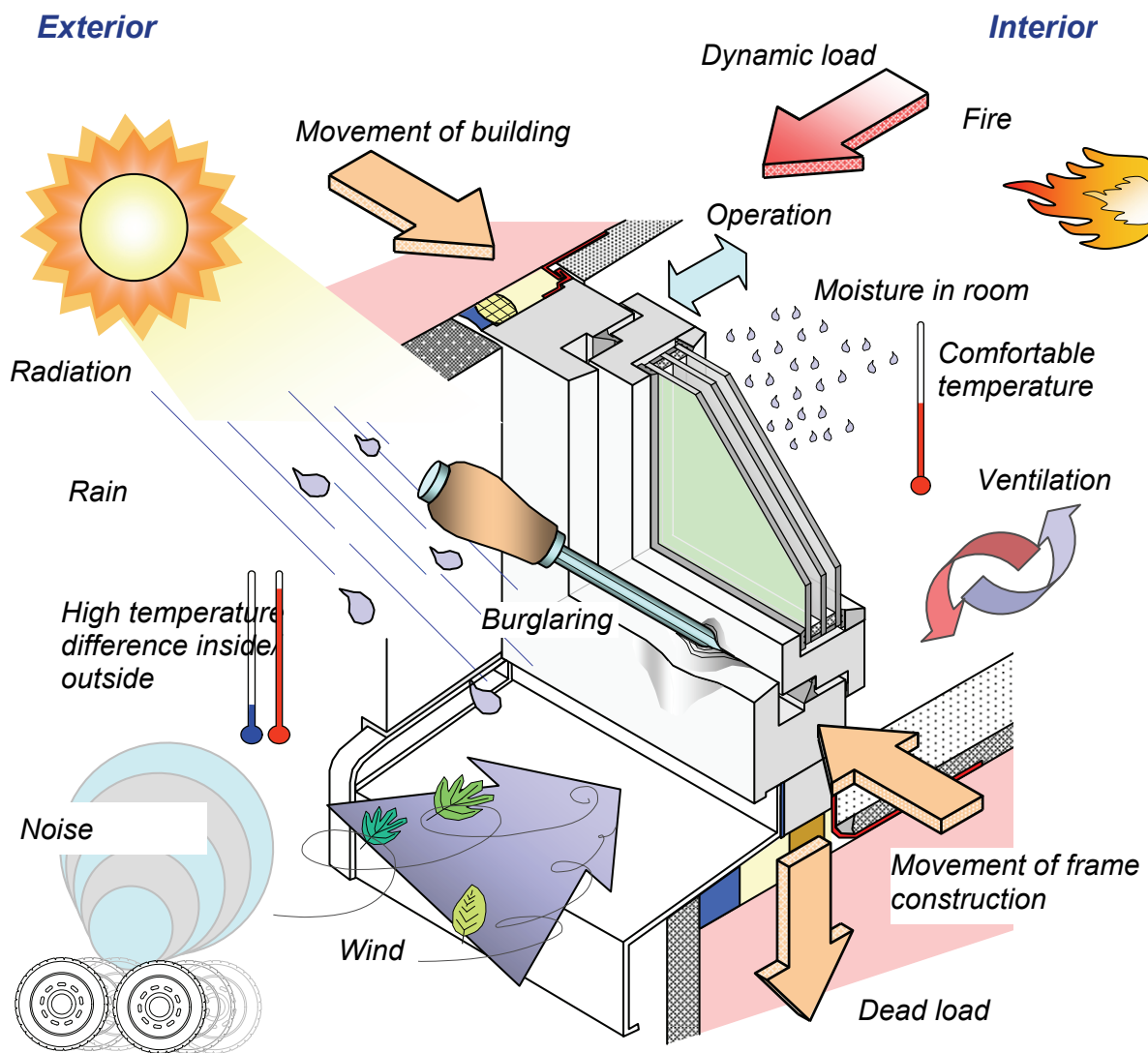
Figure 2.2 Schematic illustration of effects on windows and their joints
