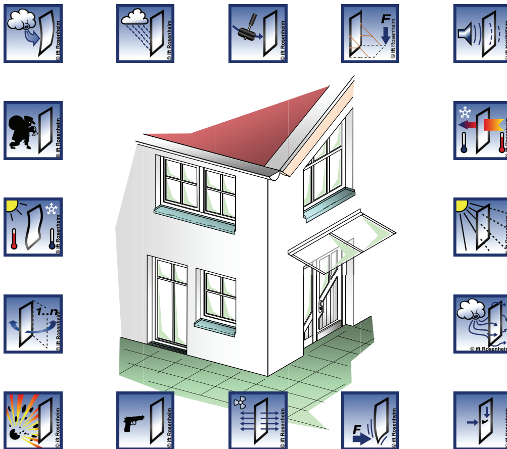
Figure 2.1 Windows and exterior doors as multifunctional building components, selected properties in accordance with Product Standard EN 14351-1
