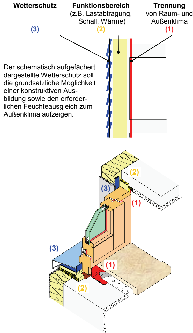
Figure 2.3 The plane model and transfer to the installation gap (applicable only conditionally to tropical/sub-tropical climatic zones).
